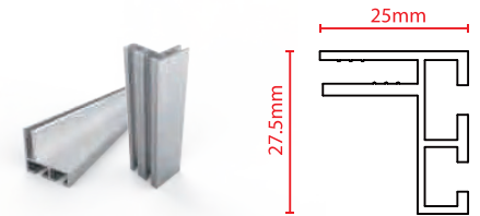
Profile Cross Section 1" (25mm)
