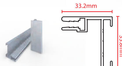
Profile Cross Section 1- 3/10" (33mm)
