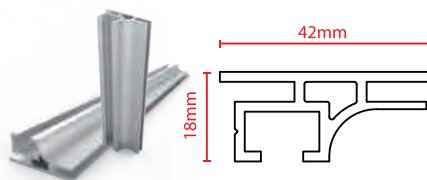
Profile Cross Section 1- 4/7" (42mm)
