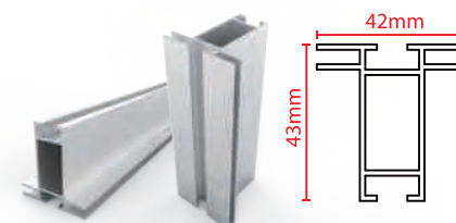
Profile Cross Section 1-13/20" (42mm)
