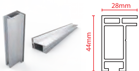
Profile Cross Section 1 1/10" (28mm)
